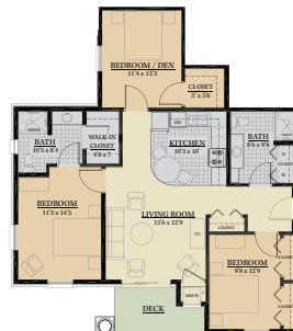
3 Bedroom A 1,206 Sq. Ft.
